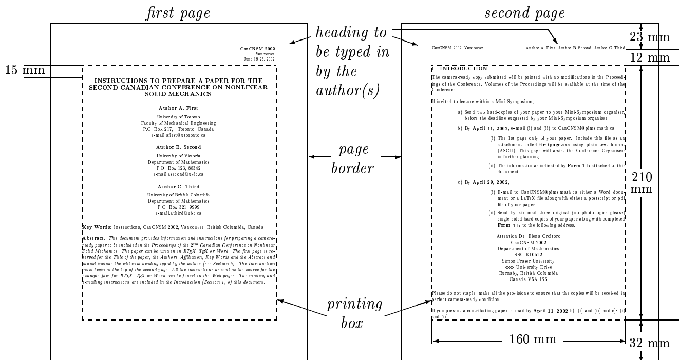
Figure 1: Page layout.
