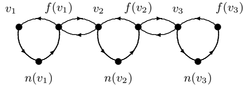
FIG. 2.1. The “next” and “former” permutations
