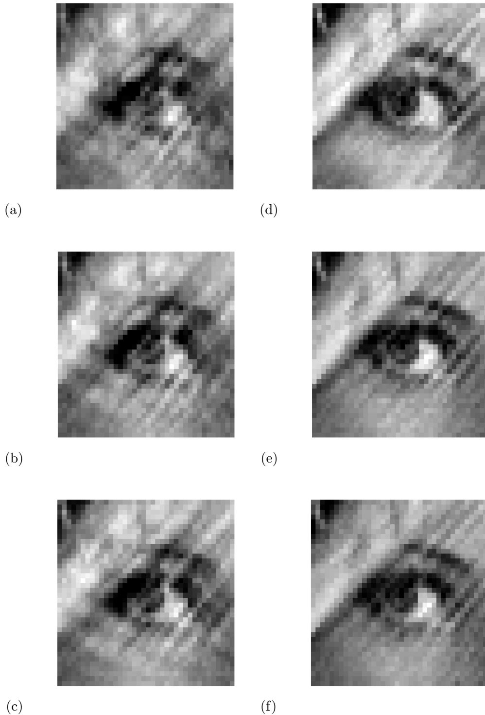
Figure 10: Typical images recovered by the HIO ( \beta = 1 ) and HPR ( \beta = 1 ) algorithms with noise (SNR=34 dB) for the data corresponding to Figure 1(d) and the normalized zero-phase initial guess shown in Figure 1(c). (a), (b), and (c) are reconstructed with 100, 200, and 400 iterations of the HIO algorithm, respectively; (d), (e), and (f) are reconstructed with 100, 200, and 400 iterations of the HPR algorithm, respectively.
